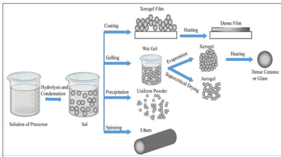
Figure 12. Different sol-gel process steps to control the final morphology of the product. Reproduced from Ref. [210] with permission from Elsevier Ltd. Iranian Chemical Society.
