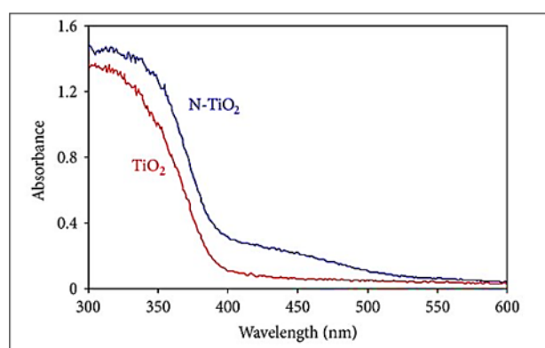
Figure 6. Ultraviolet-visible absorption spectrum of TiO 2 and N-TiO 2 . Reproduced from Ref. [175] with permission from WILEY-VCH.
