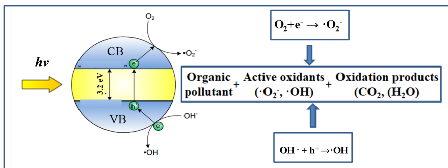
Figure 19. Scheme of formation of OH · , and O 2 ·- particles on the surface of TiO 2 under the action of light.
