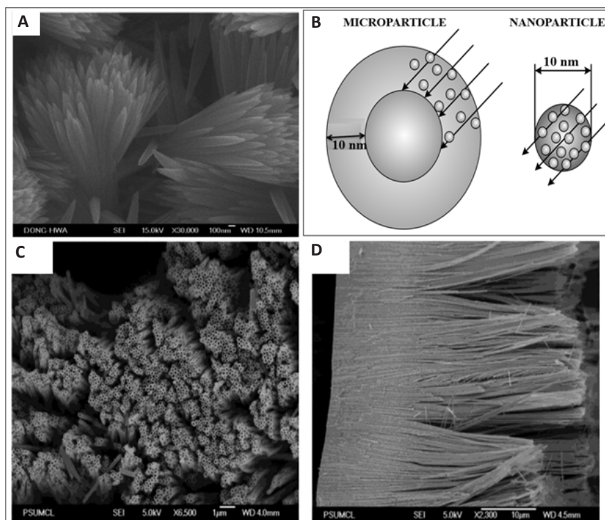
Figure 14. (A) An FESEM image of TiO 2 nanorods in Mali's work. Reproduced from Ref. [245] with permission from Royal Society of Chemistry; (B) absorption of light quanta in TiO 2 micro- and nanoparticles. Reproduced from Ref. [190] with permission from Pleiades Publishing, Ltd.; Microphotographs of the TiO 2 coating obtained by anodizing titanium in a fluoride-containing electrolyte: (C)-surface, (D)-slip [256].
