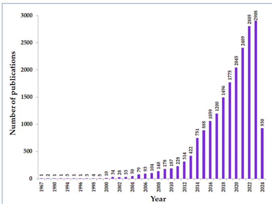
Figure 17. Annual statistics of scientific publications on photocatalysis.
