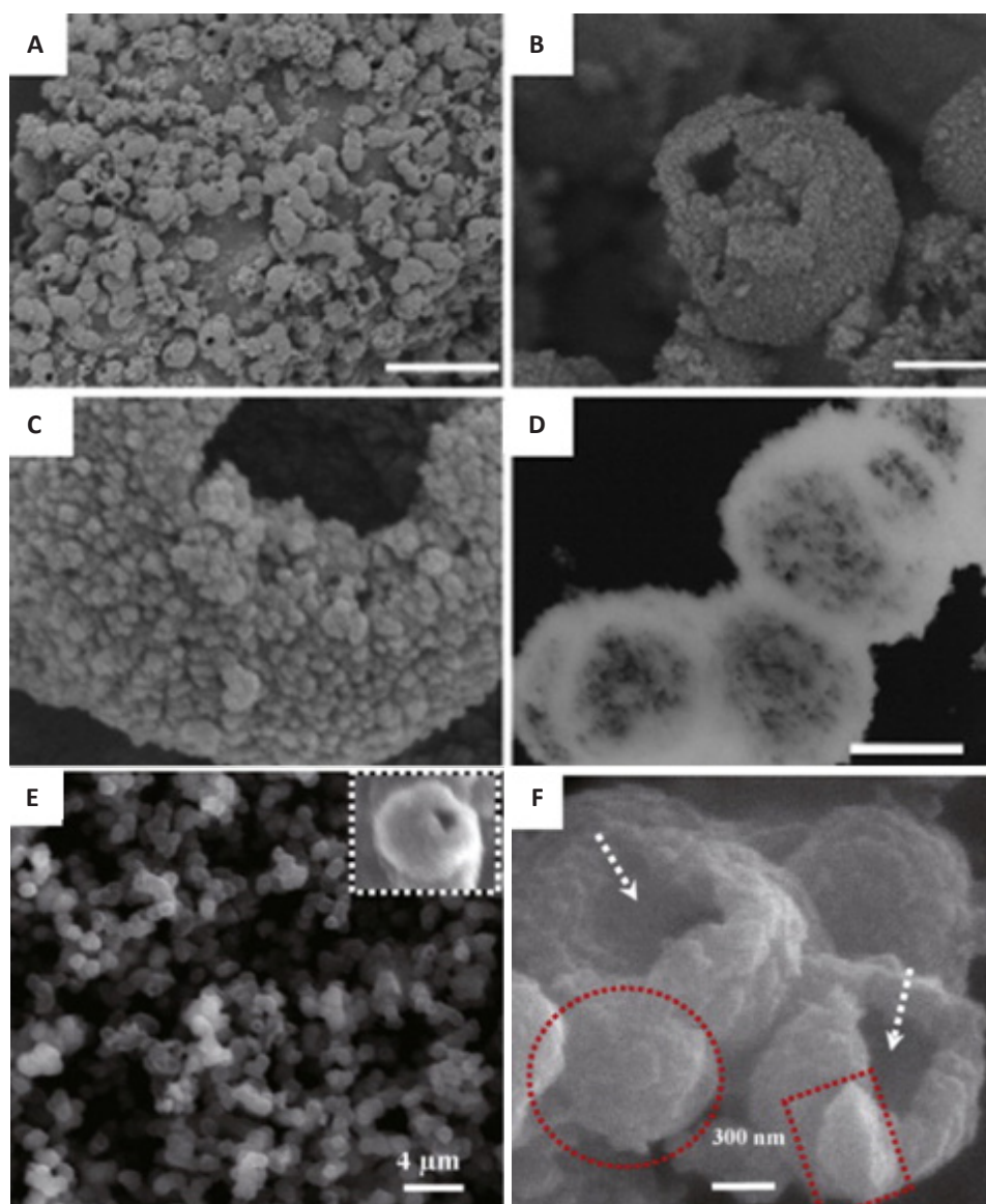
Figure 7. (A-C) FESEM and (D) TEM images of the porous, hollow TiO 2 aggregates prepared by the hydrothermal treatment at 160°C for 6 h. Reprinted with permission from [187] , Copyright © 2007 WILEY-VCH Verlag GmbH & Co. KGaA, Weinheim; (E, F) SEM overviews of the TiO 2 hollow spheres synthesized by the hydrothermal method at 423K for 10h. The scale bars for (A-D) are 5mm, 500nm, 100nm, and 500nm, respectively. Reproduced from Ref. [186] with permission from Elsevier B.V.
