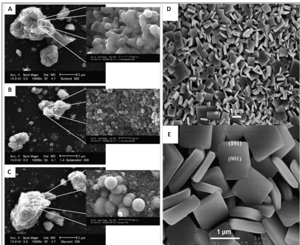
Figure 8. (A-C) SEM images for the TiO 2 prepared by the solvothermal method in various alcohol solutions: (A) 300°C, butanol, (B) 300°C, 1,4-butanediol, and (C) 300°C, glycerol. Reproduced from Ref. [191] with permission from Korean Institute of Chemical Engineering; (D, E) SEM images of the anatase TiO 2 nanosheets synthesized with a reaction time of 11h. Reproduced from Ref. [192] with permission from American Chemical Society.
