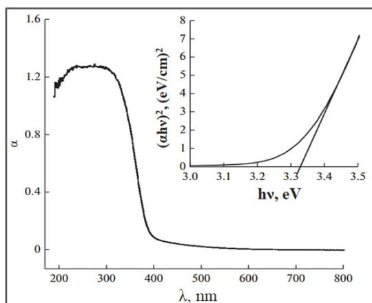
Figure 5. Absorption spectrum of TiO 2 with anatase structure.
