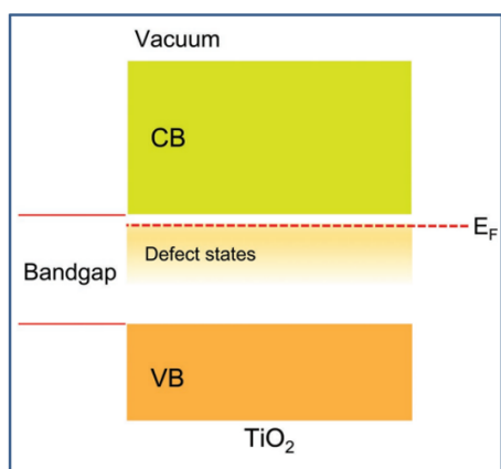
Figure 3. Schematic diagram of the electronic structure of TiO 2 . Reproduced from Ref. [159] with permission from WILEY-VCH Verlag GmbH & Co. KGaA, Weinheim.
