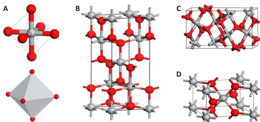
Figure 2. Crystal structure of TiO 2 : anatase (B), brookite (C), rutile (D) during thermal treatment, anatase and brookite change to rutile at temperatures of 400-1000°C and ~ 750°C, respectively.
