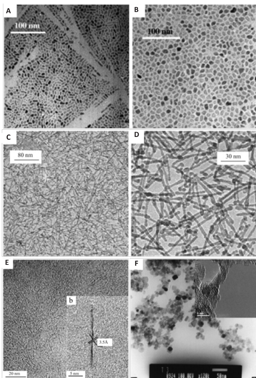
Figure 10. TEM images of TiO 2 nanoparticles (A, B) and TiO 2 nanorods (C, D). Reproduced from Ref. [187] with permission from WILEY-VCH Verlag GmbH & Co. KGaA, Weinheim; (E) TEM image of atomically thin N-TiO 2 wires grown at 180°C for 1h. Reproduced from Ref. [197] with permission from WILEY-VCH Verlag GmbH & Co. KGaA, Weinheim; (F) TEM image of as-prepared. Reproduced from Ref. [198] with permission from Elsevier B.V.
