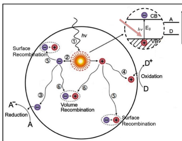
Figure 16. Pathways of the photogenerated charge carriers in a semiconductor photocatalyst. Reproduced from Ref. [159] with permission from WILEY-VCH Verlag GmbH & Co. KGaA, Weinheim.
