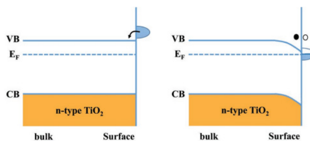
Figure 4. Scheme of surface band bending on a clean TiO 2 surface under vacuum conditions, induced by the donor - like surface defect states (●, electron; ○, hole). Reproduced from Ref. [159] with permission from WILEY-VCH Verlag GmbH & Co. KGaA, Weinheim.
