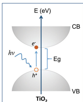
Figure 15. Schematic diagram of a typical excitation of electrons from the filled TiO 2 VB to the unoccupied CB via band-to-band excitation. Reproduced from Ref. [159] with permission from WILEY-VCH Verlag GmbH & Co. KGaA, Weinheim.
