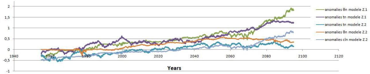
Supplementary Figure 2. Graphs Concerning Simulations Made On \Theta_n , T_n and Cl_n for the Period 1955-2095. Simulations of \theta_n and t_n anomalies ( ^{\circ}C ) obtained with the Z.1 model. (respectively green and purple curve). Simulations of \theta_n , t_n anomalies ( ^{\circ}C ) obtained with the Z.2 model (respectively orange curve and blue curve). Simulations of cl_n anomalies (%) obtained with the Z.2 model (light blue curve).
