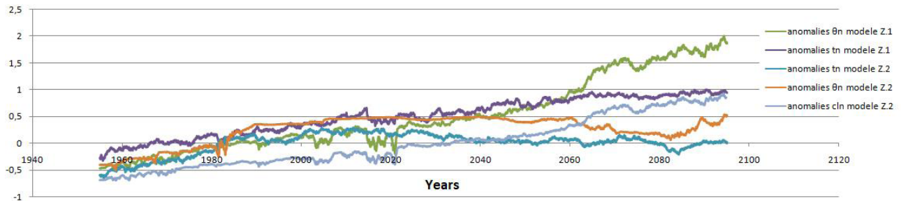
Supplementary Figure 1. Graphs Concerning Simulations Made on \Theta_n , T_n And Cl_n for the Period 1955-2095. Simulations of \theta_n and t_n anomalies ( ^{\circ}C ) obtained with the Z.1 model. (respectively green and purple curve). Simulations of \theta_n and t_n anomalies ( ^{\circ}C ) obtained with the Z.2 model (respectively orange curve and blue curve). Simulations of cl_n anomalies (%) obtained with the Z.2 model (light blue curve).
